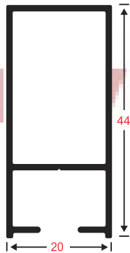
2009 JAMBA
